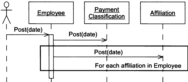
Figure 19-33 Dynamic Model Scenario: Posting Payment
